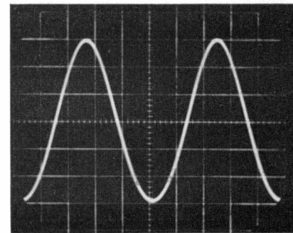
Fig. 2. Oscillograms of modulation envelope obtained when new generator was 30% amplitude-modulated by 10 kc sine wave at carrier of 1,000 Mc.
