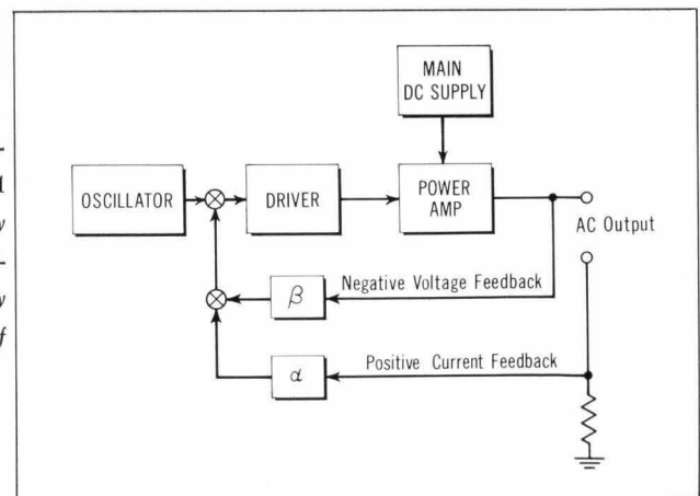
Fig. 2. Block diagram of -hp- 4301A Variable Frequency Power Supply. External signal may be used in place of oscillator signal.
