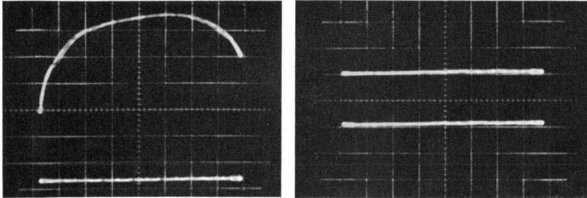
Fig. 9. Oscillograms of detected power output when FM-modulating showing advantage of automatic leveling (right)
