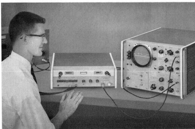
Fig. 1. New -hp- Model 8614A Signal Generator operates from 800 to 2400 Mc and provides outputs up to 10 to 60 mw. Generator is designed to provide leveled output, is also capable of being sine-wave modulated.
