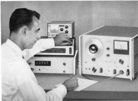
Fig. 1. Hewlett-Packard Model 4301A Variable Frequency Power Supply furnishes up to 250 volt-amperes at frequencies from 40 to 2000 cps. Output voltage is continuously adjustable from 0 to maximum of 130 or 260 volts. Unit also can serve as excellent line isolator.
